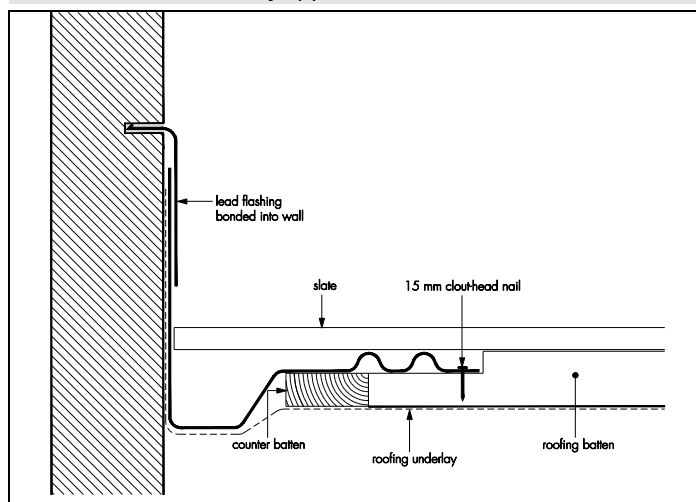
Figure 2 Filon GRP Abutment Secret Gutter/Soaker (GAS 1) with slate roof application
