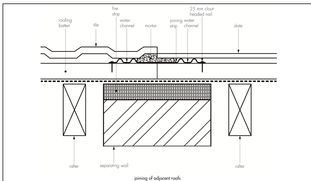
Figure 1 Filon GRP Secret Joining Strip (GJS 1)
