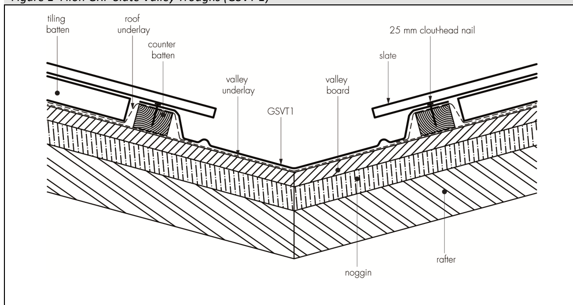
Figure 1 Filon GRP Slate Valley Troughs (GSVT 1)
